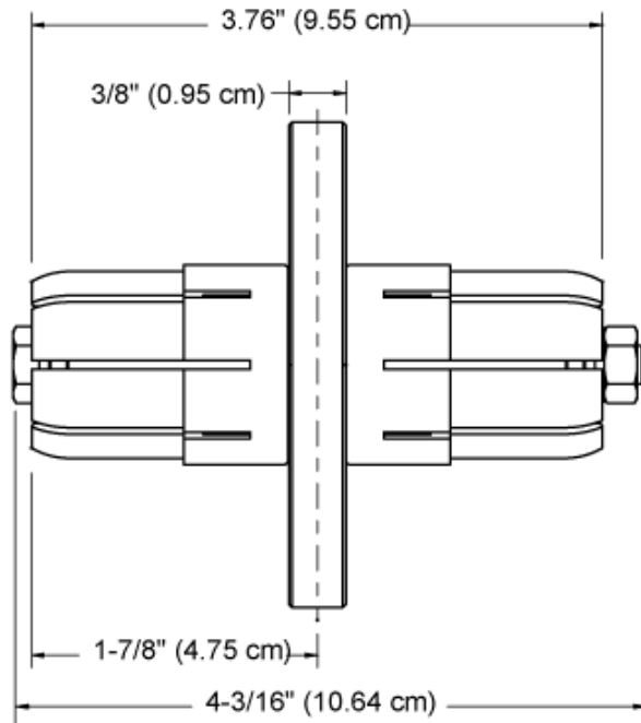
3-1/8" Anchor Connector For Flanged Line Part No. 318F-5
